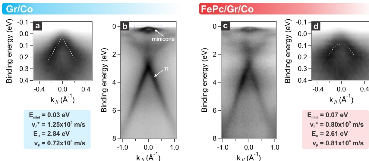
Figure 1. Comparison of the energy vs. momentum maps acquired at the \bar{K} point ( h\nu = 40 \text{ eV} ) before (a and b) and after (c and d) deposition of FePc on Gr/Co. b) and c) present the full energy region comprising the main Dirac cone and the minicone. a) and d) present the zoom of the region near the Fermi level where the minicone state is located. The corresponding values of Fermi velocity and the energy position of the maximum of minicone ( v_F^* , E_{\text{mini}} ) and Dirac cone ( v_F , E_D ) are given in blue and red boxes for pristine Gr/Co and FePc/Gr/Co, respectively.
